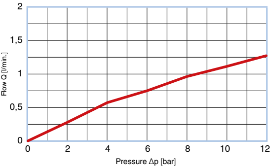
CHECK VALVE® Flow curve – screened BF660080024100; T = 50 °C, hydraulic oil HLP46
