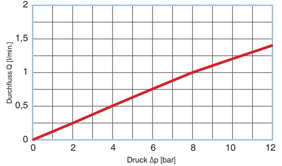
CHECK VALVE® Flusskurve – screened BFAA055014; T = 50 °C, Hydrauliköl HLP46
