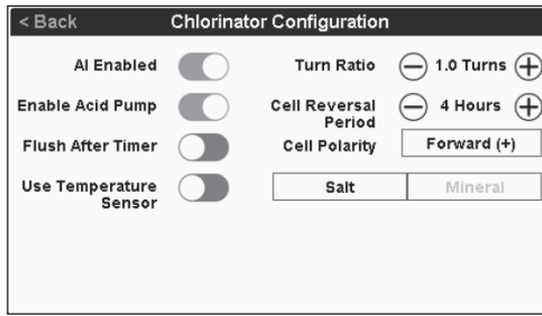
Figure 5. Select Saltwater or Mineral Water
