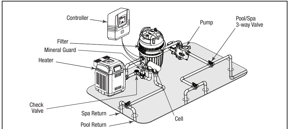
Figure 3. Typical Installation Diagram
