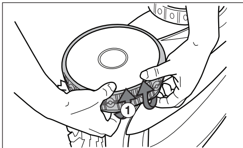
Figure 23. Pull the Old Tyre Over the Wheel
