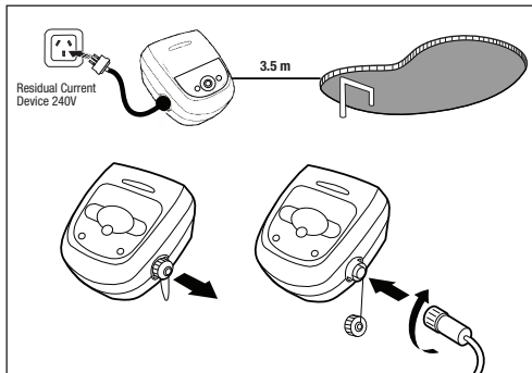
Figure 3. Connect/Disconnect the Floating Cable
