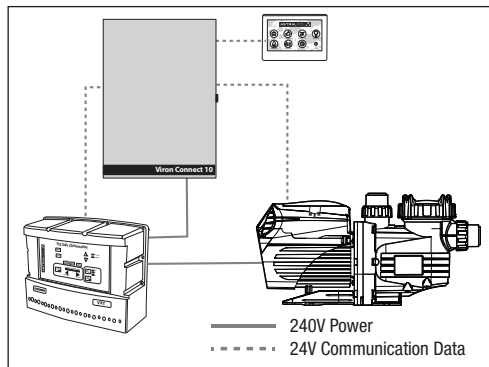
Figure 28. Viron XT Series 2 Pump, VX S (Non-timer Model) Chlorinator and Viron Connect 10 Remote Control System
