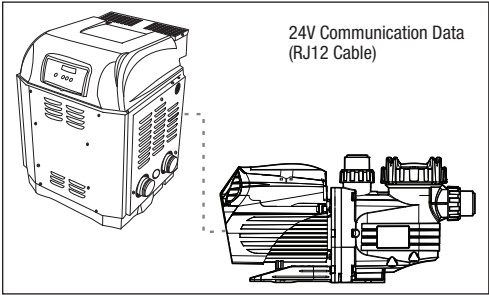
Figure 29. Viron XT Series 2 Pump with RJ12 Cable Connection
