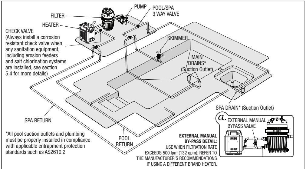
Figure 8. Typical Water Piping Configuration
