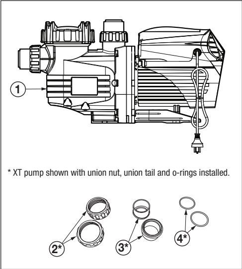
Figure 3. Viron XT Series 2 Pump Components
