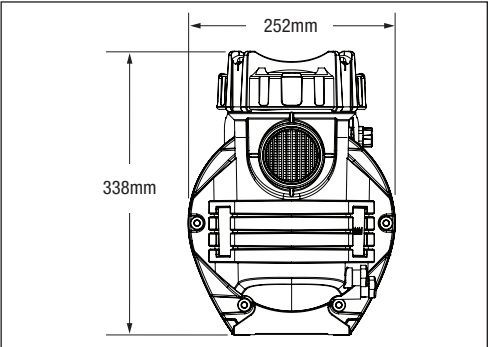
Figure 1. Front Dimensions
