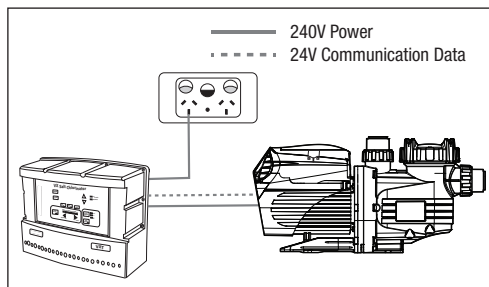
Figure 27. Viron XT Series 2 Pump, Compatible VX Timer Model Chlorinator and Remote Control
