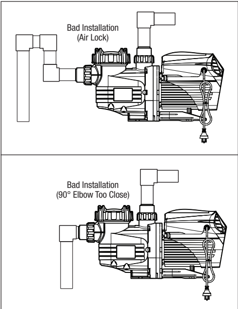
Figure 5. Viron XT Series 2 Pump Incorrect Piping Installations
