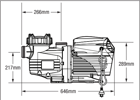
Figure 2. Side Dimensions
