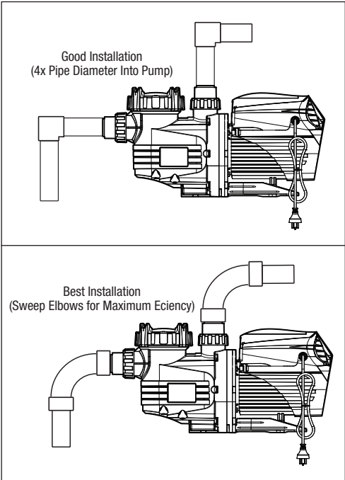
Figure 6. Viron XT Series 2 Pump Good Piping Installations
