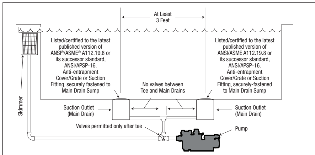
Figure 9. Number of Suction Outlets Per Pump
