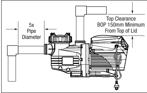
Figure 7. Viron XT Series 2 Pump Piping Clearance
