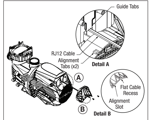
Figure 10. Data Port Location on XT Pump
