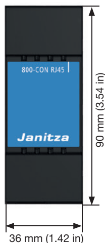
Vista frontal
