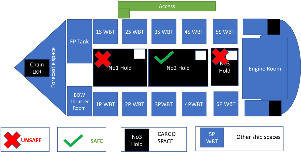
Example of a simplified diagram to be placed at the ship's access point to assist shore personnel in identifying safe and unsafe spaces on board the ship.
