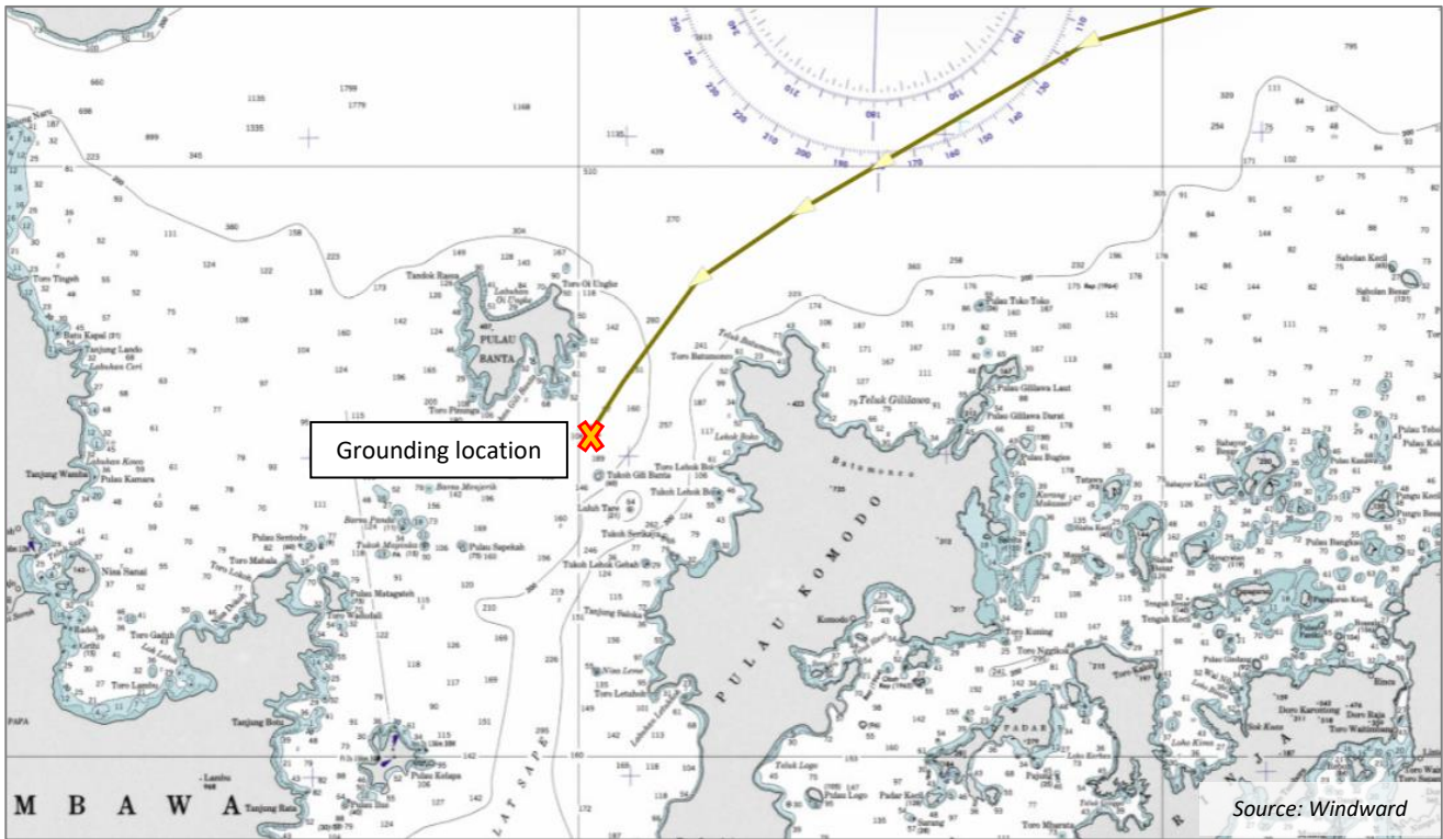
AIS track of the vessel in case study 3
