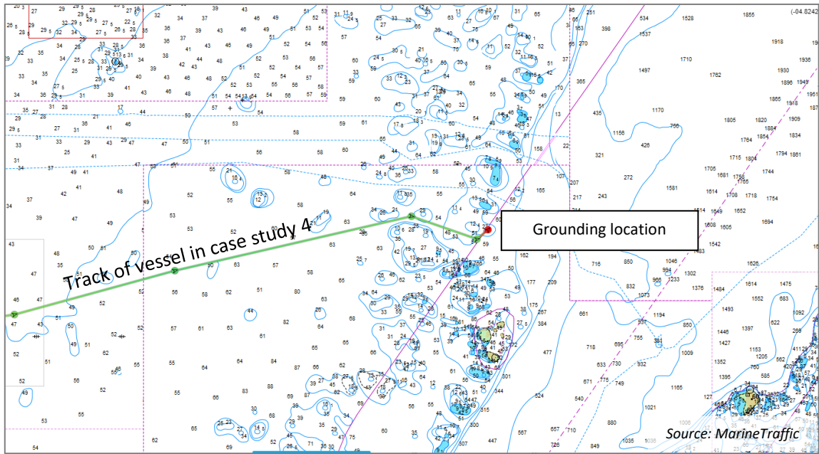
Close up of the area where the vessel grounded on an uncharted obstruction
